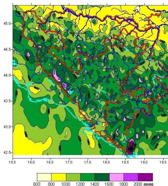
Figure 1.4.2.: Spatial distribution of mean annual precipitation in BH, 1961-1990.
