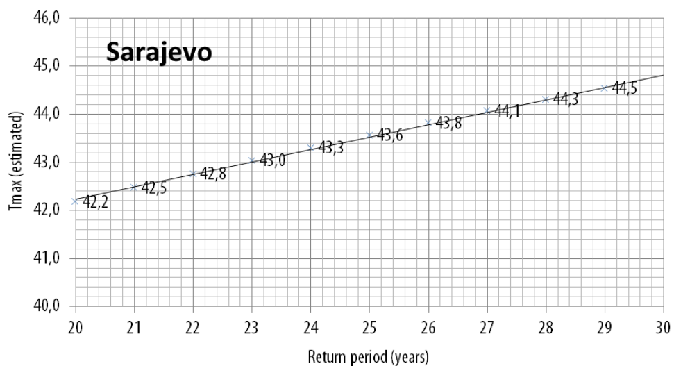
Fig. 3.2.13 Projected maximum annual temperatures of air in Sarajevo for return period of 20 – 30 years
