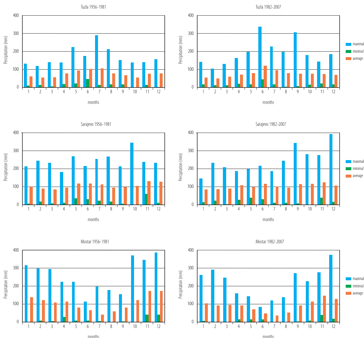
Figure 3.4.2.1 Extreme and average values for monthly precipitation in Tuzla, Sarajevo and Mostar for the periods 1956–1981 and 1982–2007.
