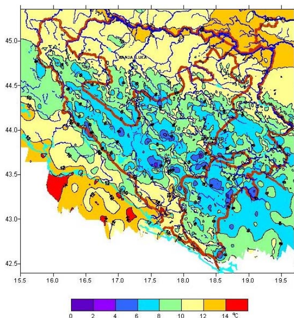
Figure 1.4.1.: Spatial distribution of mean annual air temperature in BiH, 1961-1990.
