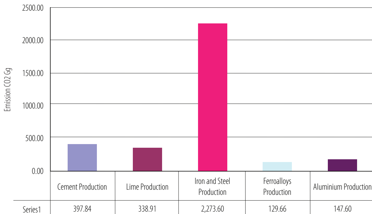
Figure 2.4.3. 1.: Sectoral report for industrial processes
