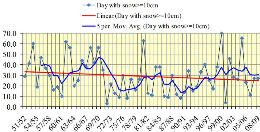
Fig. 3.2.11 Annual number of days with snow cover \geq 10 cm in Sarajevo (1951–2007).
