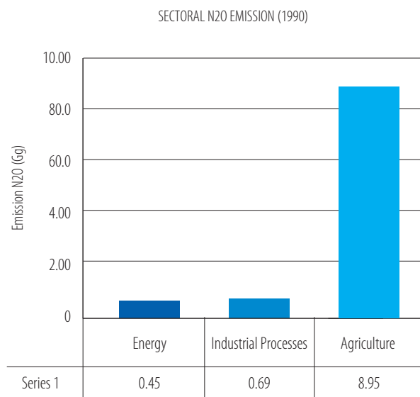
Figure 2.4.6.1.: Sub-nitrogen emissions by sector (N 2 O) (1990).
