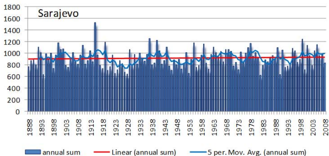
Fig. 3.2.8 Annual total rainfall in Sarajevo, 1888-2008.
