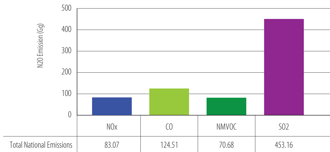
Figure 2.5.1.: Total emission of indirect greenhouse gases (1990).
