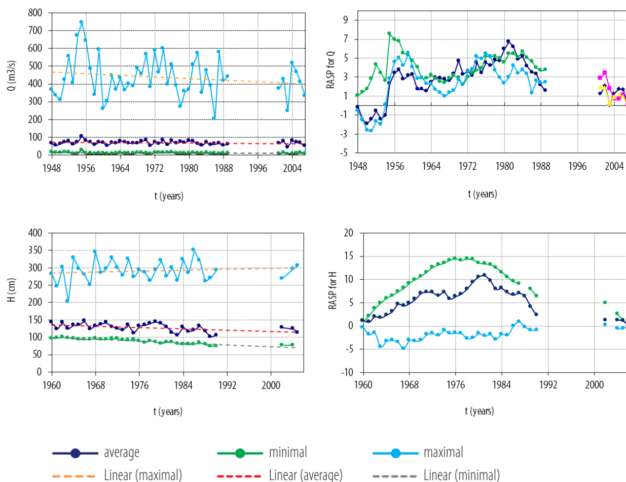
Fig.3.4.2.2. Maximum, average and minimum discharges and RAPS parameter for the Sana River in Sanski Most in the period 1948-2007 (top row) and maximum, average and minimum water levels and RAPS parameter for the Buna Rivers near Buna in the period 1960-2006 (bottom row).
