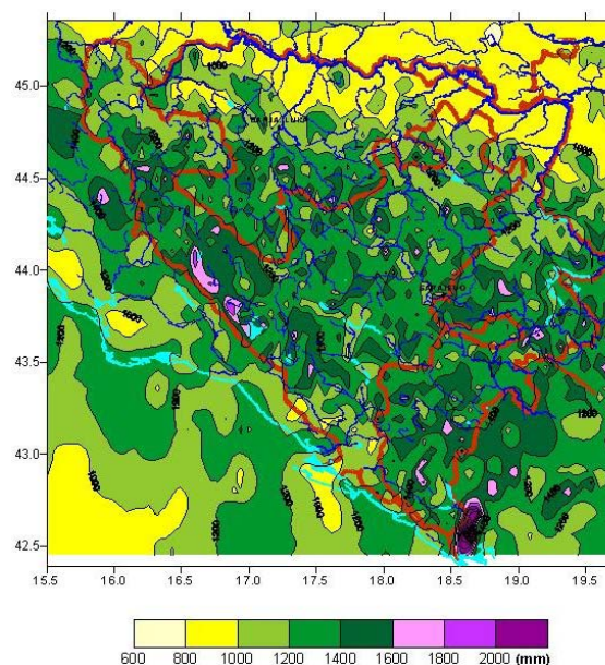
Fig. 3.1.2 spatial distribution of mean annual rainfall in BiH, 1961–1990.
