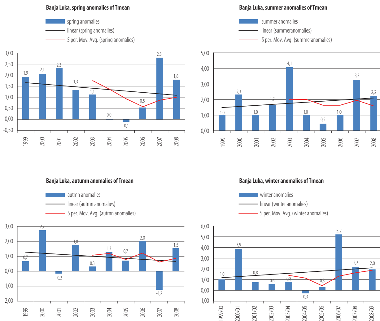
Fig. 3.2.4 Seasonal air temperature anomalies in Banja Luka, 1999–2008. 10
