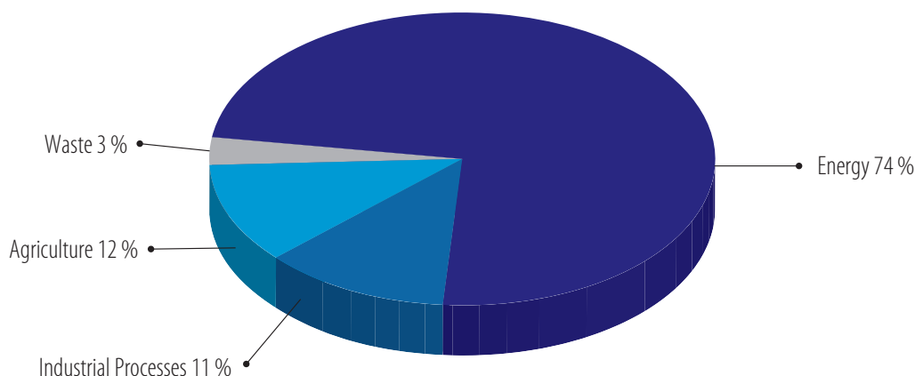
Figure 2.4.1.2.: Share of CO 2 e emissions by sector.
