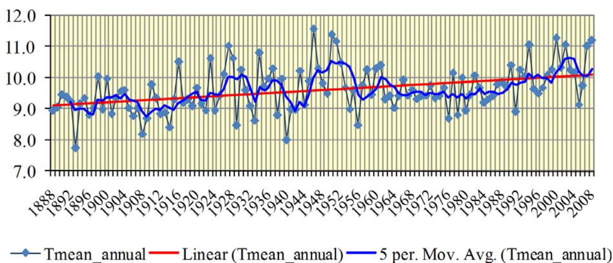
Fig. 3.2.2 Average annual temperature in Sarajevo, 1888–2008.
