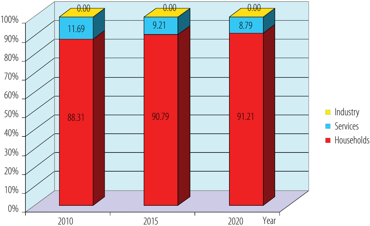
Picture 4.2.5.2.2.: Reduction in final energy consumption (S3-S2) by sector in RS
