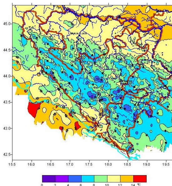
Fig 3.1.1 spatial distribution of mean annual air temperatures in BiH, 1961–1990.
