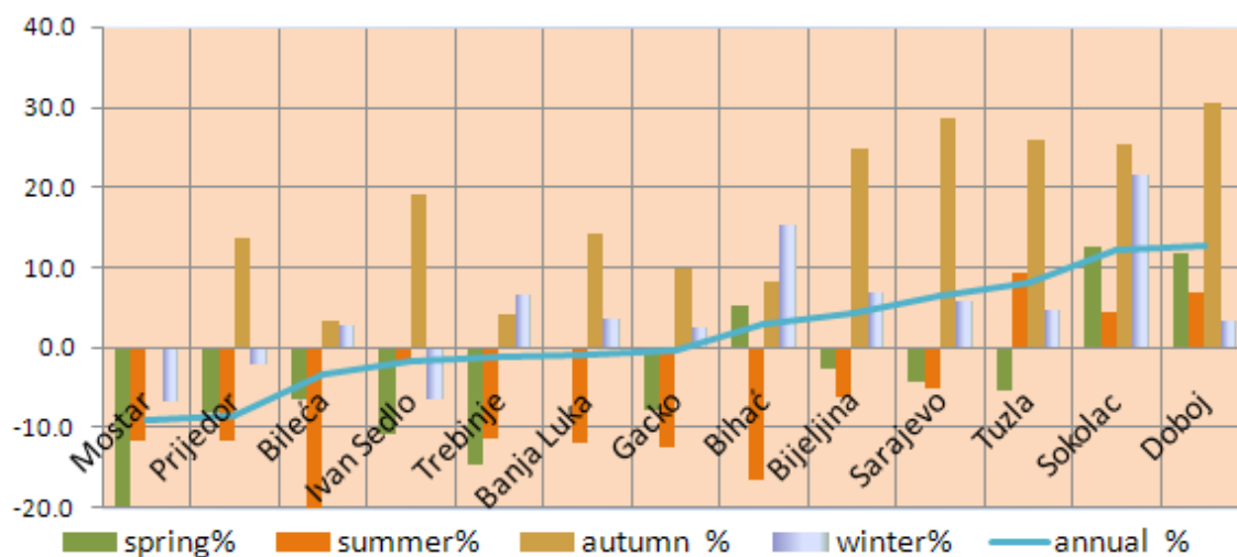
Fig. 3.2.7 Surplus/deficit of rainfall as a percentage of total average annual of rainfall in the last decade (1999-2008) compared to the reference period (1961-1990). 11
