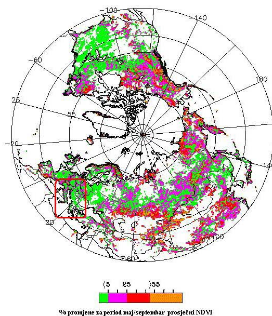
Fig. 3.4.1.3.1. Increase in the NDVI for the period May–September (1982–1990).
