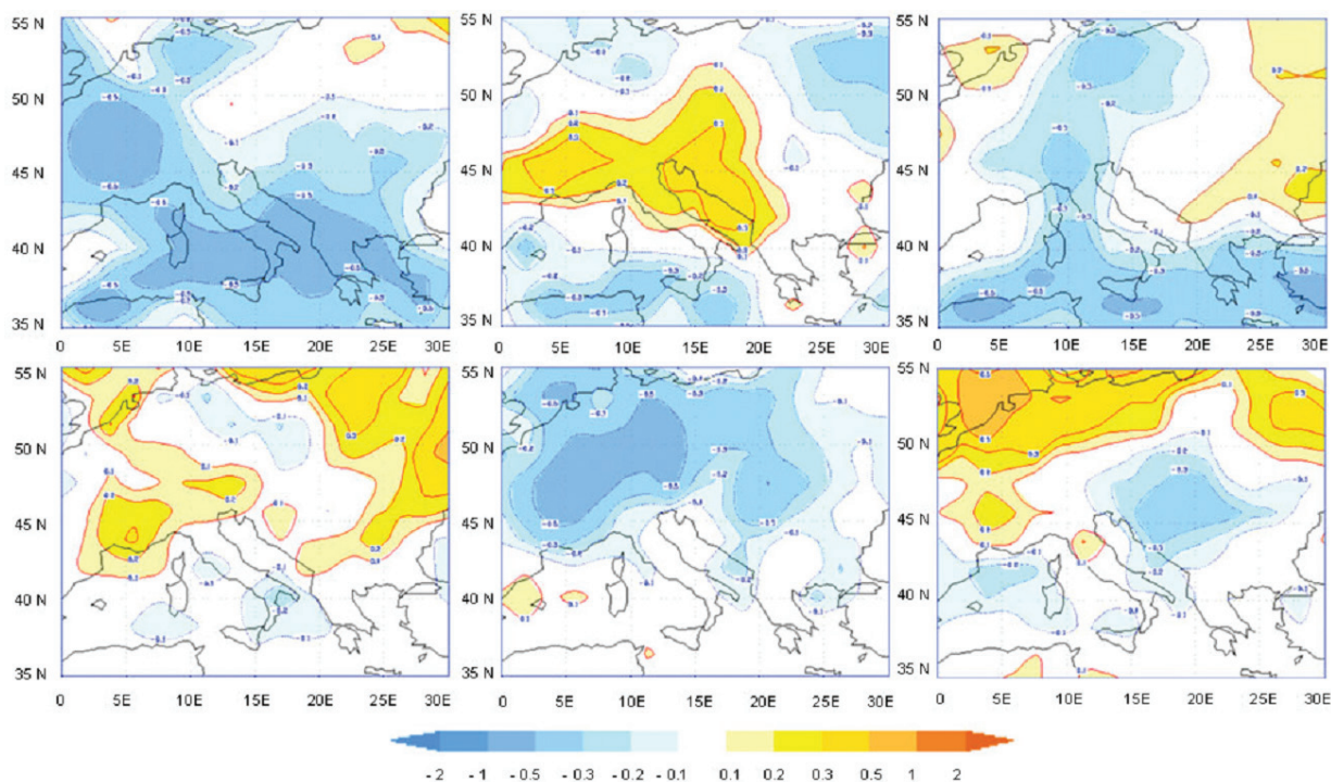
Fig. 3.2.1 Represents the climate of the 20th century better than the last decade of the 20th century and 2040–2050
