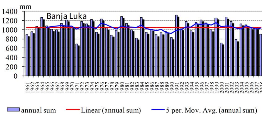
Fig. 3.2.9 Annual total rainfall in Banja Luka, 1961-2008.
