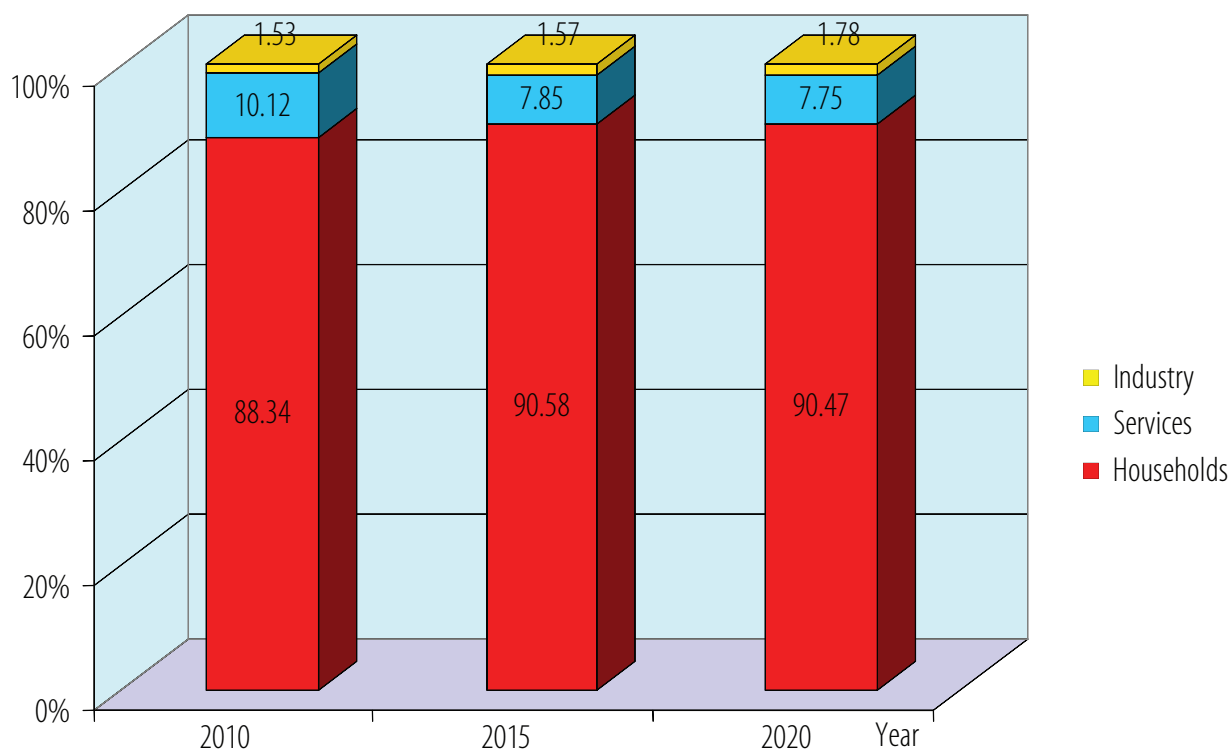
Picture 4.2.5.2.3.: Reduction in final energy consumption (S3-S2) by sector in BiH
