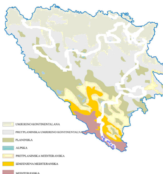
Fig. 3.1.3 Types of climate in BiH.
