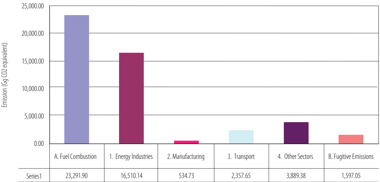
Figure 2.4.2.2.: Energy sector – summary report for CO2 equivalent emission 1990 year
