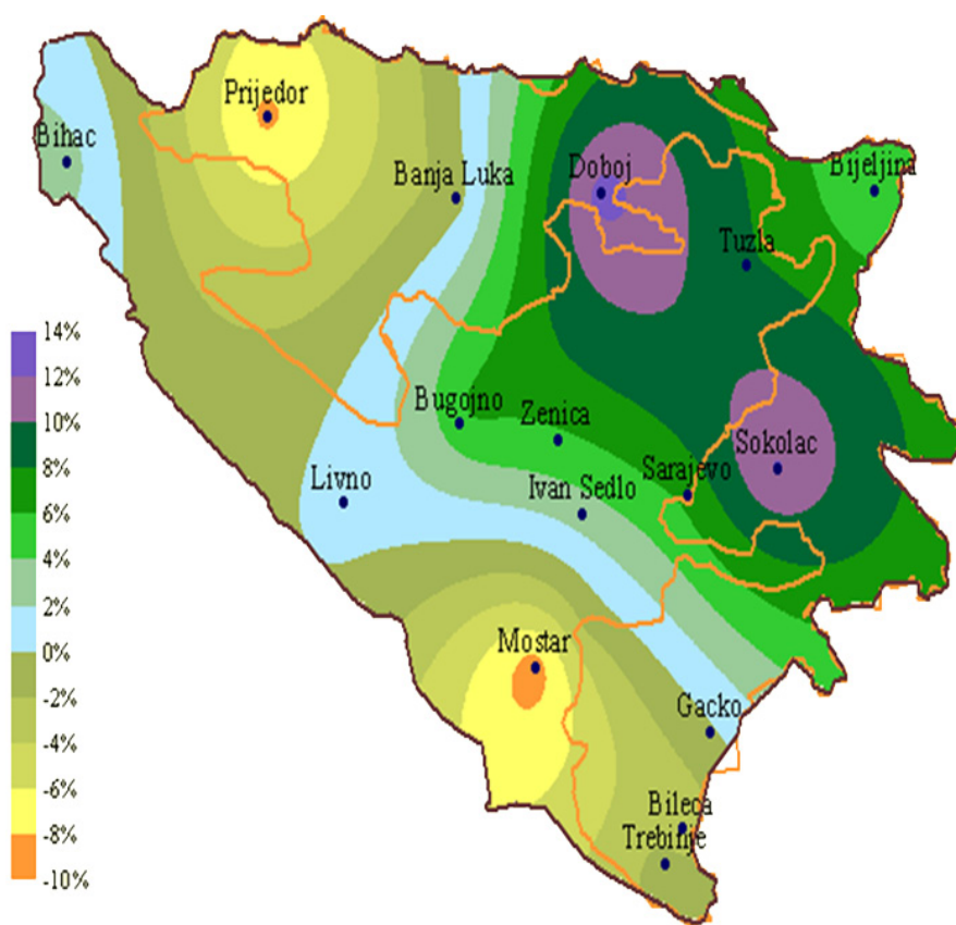
Fig. 3.2.6 spatial distribution of annual surplus/deficit of rainfall in the last decade (1999–2008) compared to the reference period (1961–1990) of BiH.
