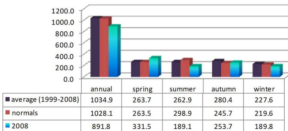
Fig. 3.2.10 Seasonal precipitation. Comparison of the past decade, the reference period, and the year 2008.
