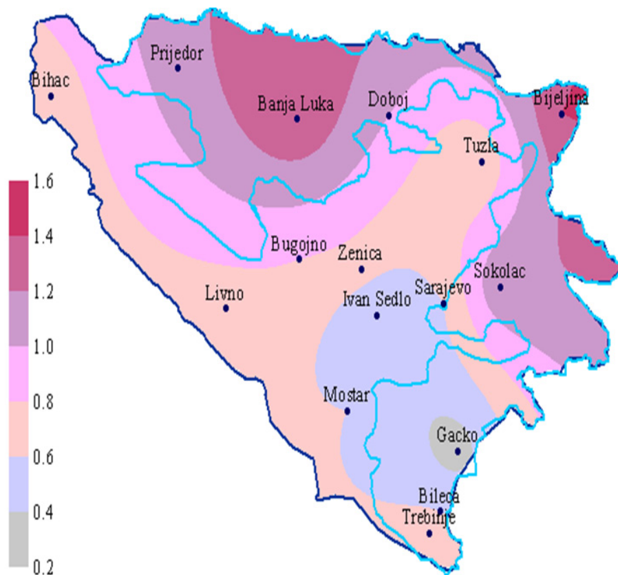
Fig. 3.2.5 Increase in average annual temperature in the last decade (1990–2000) compared to the reference period (1961–1990) in BiH expressed in °C.
