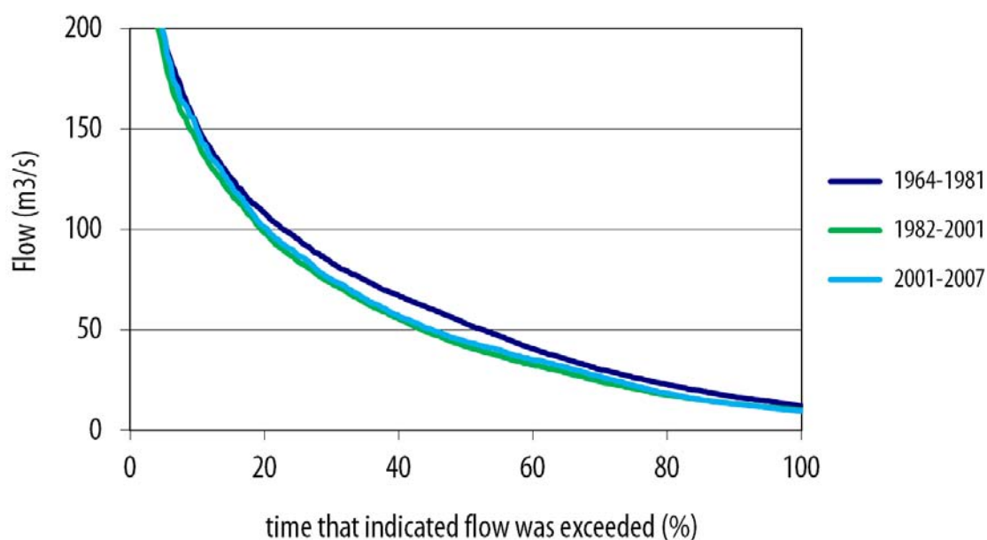
Figure 3.4.2.3. Flow-duration curve for different periods, Sana River in Sanski Most.
