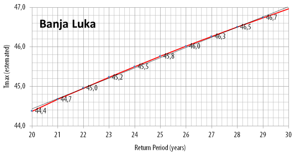
Fig. 3.2.12 Projected maximum annual temperatures of air in Banja Luka for the return period of 20 – 30 years
